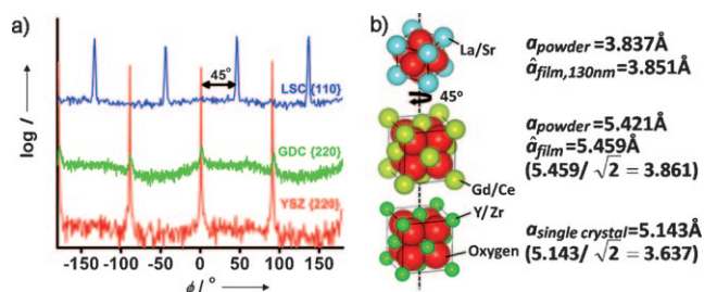
Figure 2. a) Off-normal XRD patterns of LSC 130nm //GDC/(001) cubic YSZ. b) The cube-on-cube alignment of GDC on YSZ and the 45° in-plane rotation ( \phi ) of LSC on GDC.
